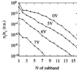
FIG. 5. Electron concentration in first 16 energy subbands (relatively to the concentration in the first subband) at different reverse biases. Sample #300 ( \Delta E_C = 175 meV), T = 300 K.
