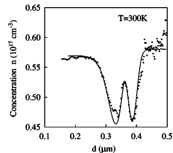
FIG. 10. Apparent concentration profile of \text{In}_x\text{Ga}_{1-x}\text{As}/\text{GaAs} quantum well with low In-content x_{\text{In}}=0.065 (dotted) and fitted curve (solid) with \Delta E_C = 55 meV (sample #298).
