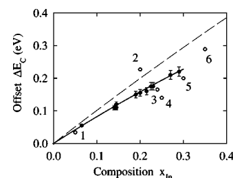
FIG. 12. Conduction band offsets in strained \text{In}_x\text{Ga}_{1-x}\text{As}/\text{GaAs} QWs as function of composition. Errors bars correspond to the 95% confidence interval. Dashed line, as recommended in Ref. 9. Open circles, the last decade results of capacitance and optical investigations on strained \text{In}_x\text{Ga}_{1-x}\text{As}/\text{GaAs} -QWs: 1, Ref. 38; 2, Ref. 14; 3, Ref. 19; 4, Ref. 18; 5, Ref. 13; 6, Ref. 11.
