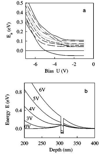
FIG. 6. Results of numerical calculations for sample #300 ( x = 0.23 ; well width = 7.2 nm; offset \Delta E_C = 175 meV); T = 300 K: (a) first 8 energy levels as function of U_{rev} ; (b) the conduction band bottom near the QW at different U_{rev} .
