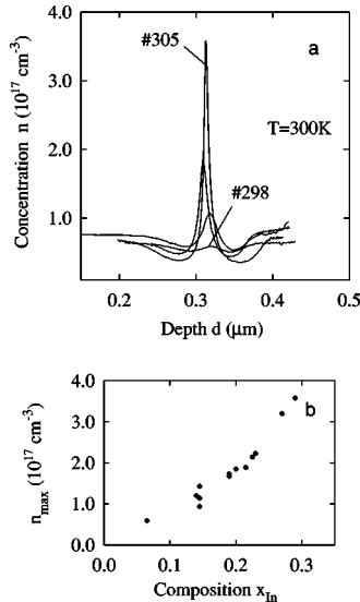
FIG. 3. C-V-profiling of \text{In}_x\text{Ga}_{1-x}\text{As}/\text{GaAs} quantum wells. Samples #296–#309. (a) Common view of apparent carrier concentrations for several samples; (b) apparent concentration peak values as a function of x . Note that near x=0.14 there are 4 samples with different width of QW.
