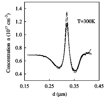
FIG. 9. Resolution of the fitting. The results for the best fit ( \Delta E_C = 120 meV, solid line) and for \Delta E_C = 130 meV (dashed line) are presented. Dotted curve, the experimental apparent profile for sample #303 ( x=0.145 ).
