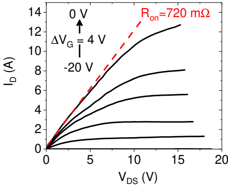
Output characteristic of an upscaled \beta\text{-Ga}_2\text{O}_3 switching transistor for converter applications.
