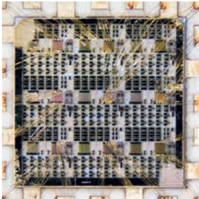
Multi-finger \beta\text{-Ga}_2\text{O}_3 switching transistor with 10 mm total gate width (left) and \beta\text{-Ga}_2\text{O}_3 chip wire-bonded on a PCB submount (right).
