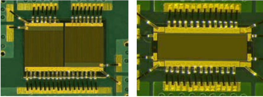
Monolithically integrated 130 mΩ/650 V half-bridge chip (left) and bi-directional transistor chip (right) on PCB submounts.
