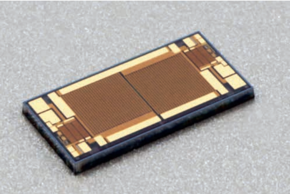
Monolithically integrated high-voltage half-bridge chip with integrated gate drivers based on the AlN-on-SiC platform.
