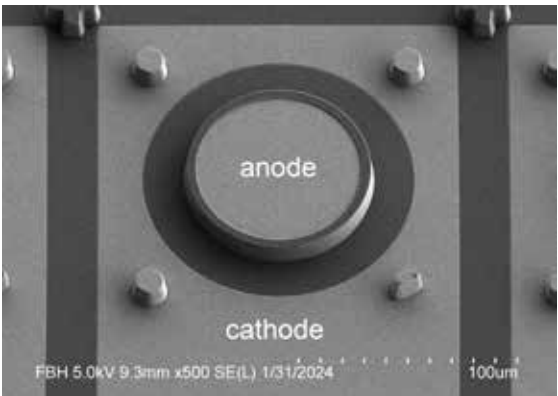
SEM picture of a processed circular quasi-vertical pn diode.
