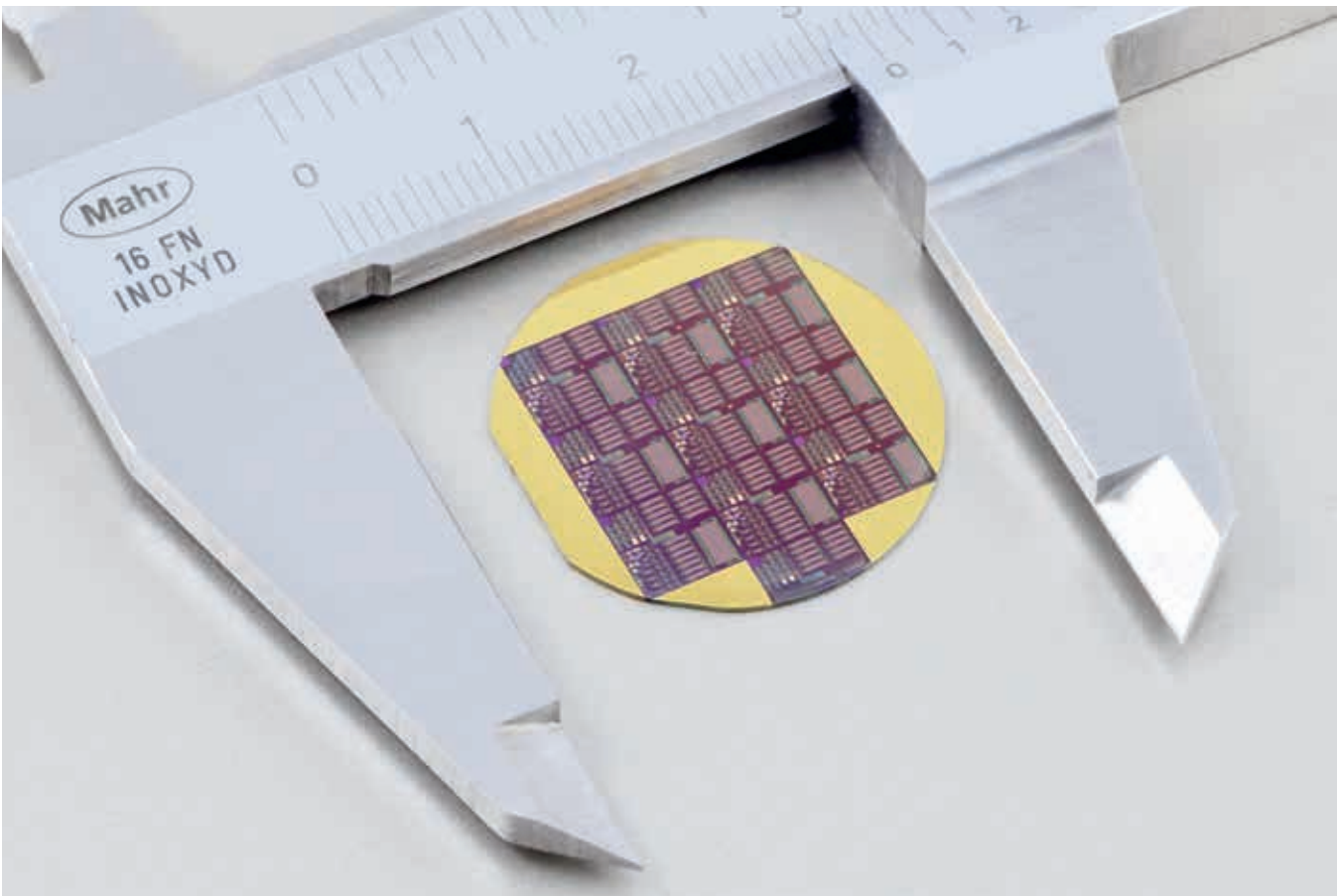
1-inch AlN-on-AlN wafer with processed power transistors.
