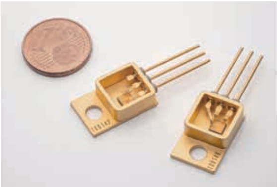
Packaged GaN trench MOSFETs on GaN substrate.
