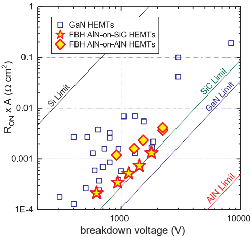
Power density benchmarking plot for lateral switching transistors based on GaN and AlN.
