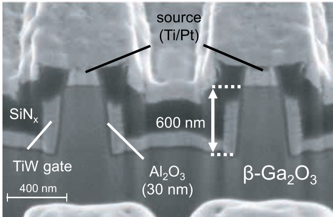
SEM cross-section image of the fully processed \beta\text{-Ga}_2\text{O}_3 FinFET device with a 1.2 \mu\text{m} pitch of the fins.
