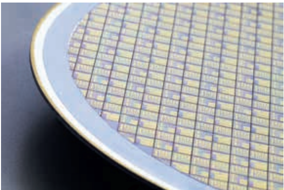
Vertical GaN Schottky diode structures after substrate transfer from 4" sapphire to tungsten.
