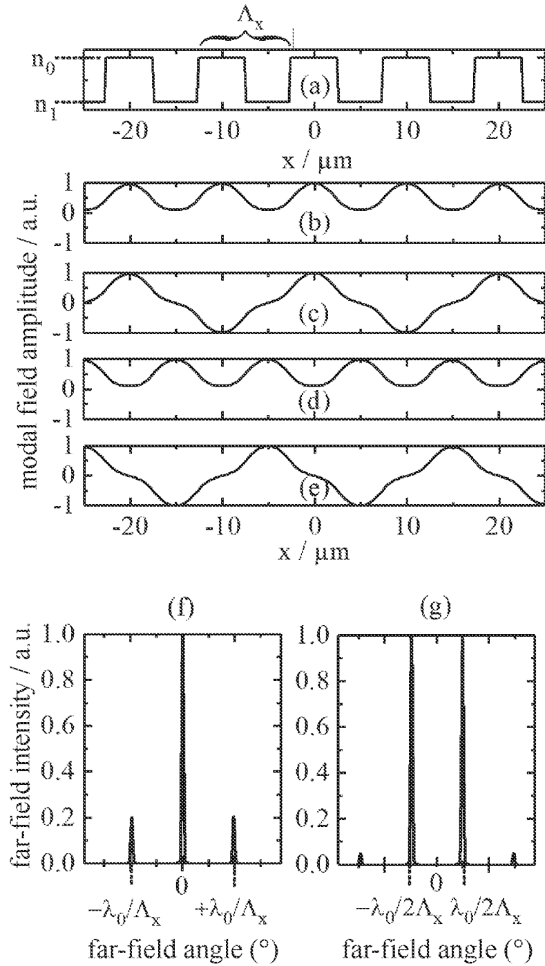
Fig. 3 (Prior Art)
