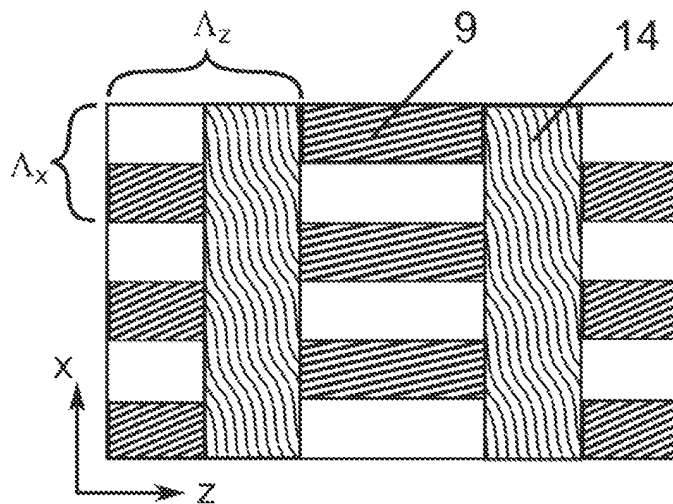
Fig. 5 (Prior Art)
