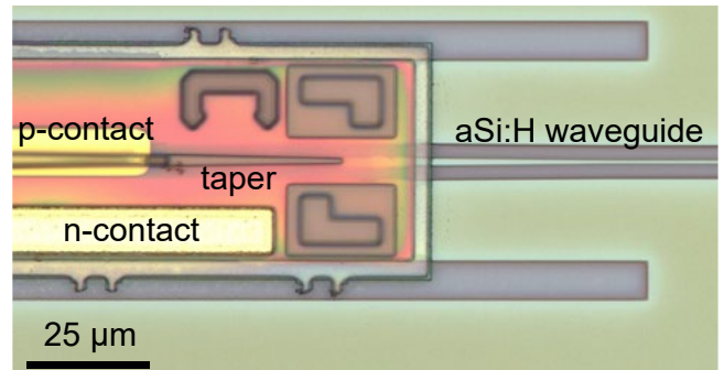
➤ Amplifier chiplet printed on intermediate waveguide.
