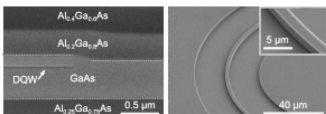
➤ SEM pictures of (left) an active-passive interface in cross section and (right) a deep-etched Euler U-bend segment in top view.
